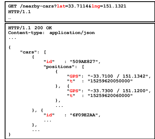
Figure 2: An example of a rider request and response message.
